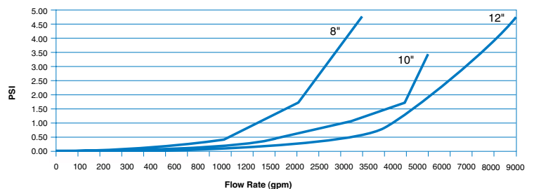
Head Loss: 8" to 12" Strainers
