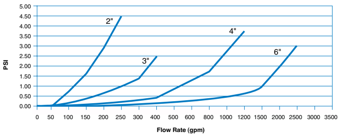
Head Loss: 2" to 6" Strainers
